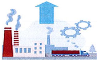
SCOP/SCOPE 1
